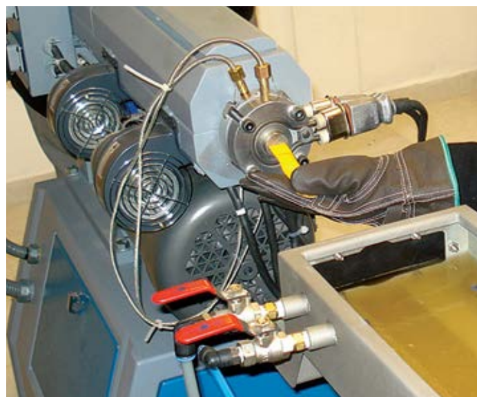
First run on extruder. Photo courtesy of Macropol.
